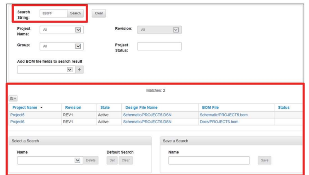
< BOM Search >
