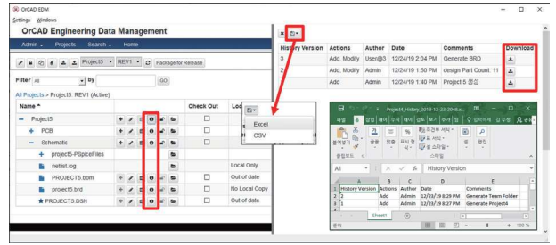
< Project History >
